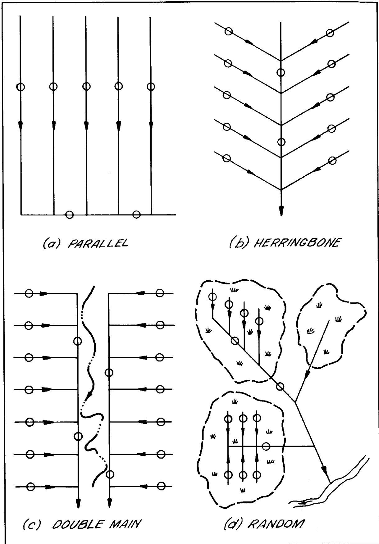
Figure 4-9, Types of drainage collection systems
