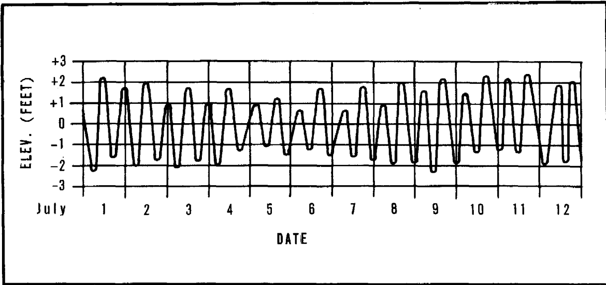
Figure 9-1, Typical ocean tide on open coastline
