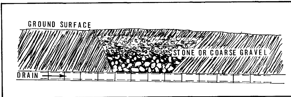
Figure 4-46, Blind inlet
