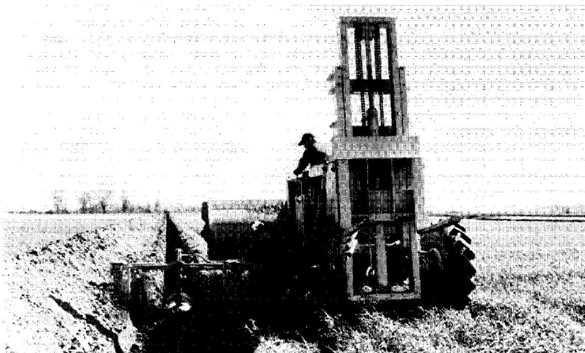
Blinding drain with machinery
