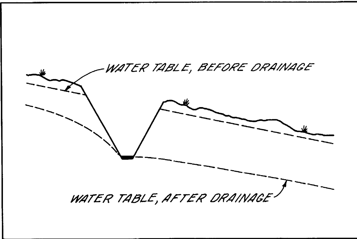
Figure 4-25a, Interception ditch
