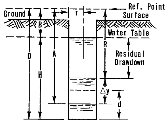
AUGER HOLE PROFILE
