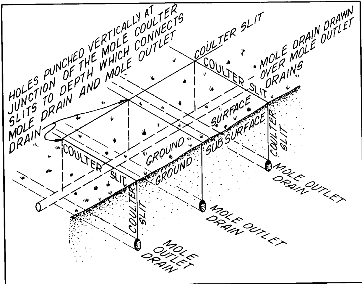
Figure 4-35, Mole drain outlets
