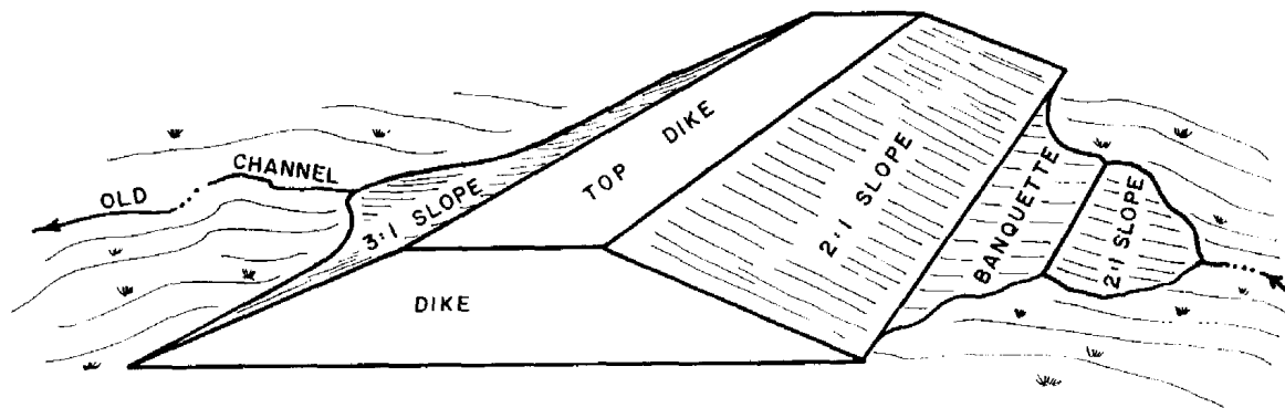
Figure 6-3, Dike section with banquette
