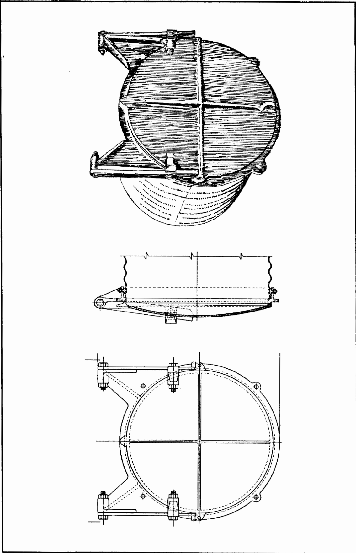
Figure 9-9, Typical low-head tide gate
