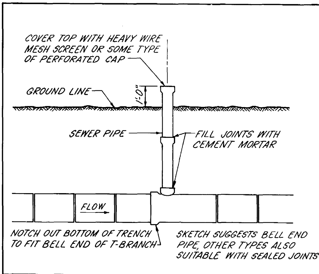
Figure 4-43, Vent
