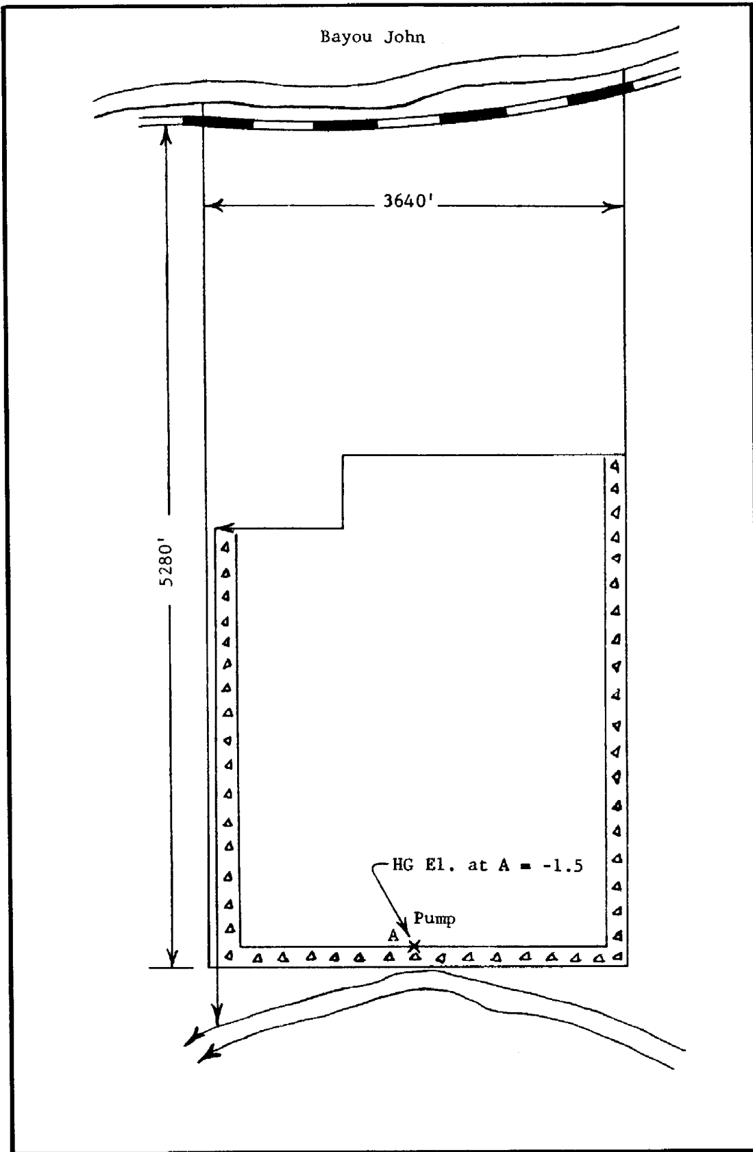
Figure 7B-1, Pump drainage site layout
