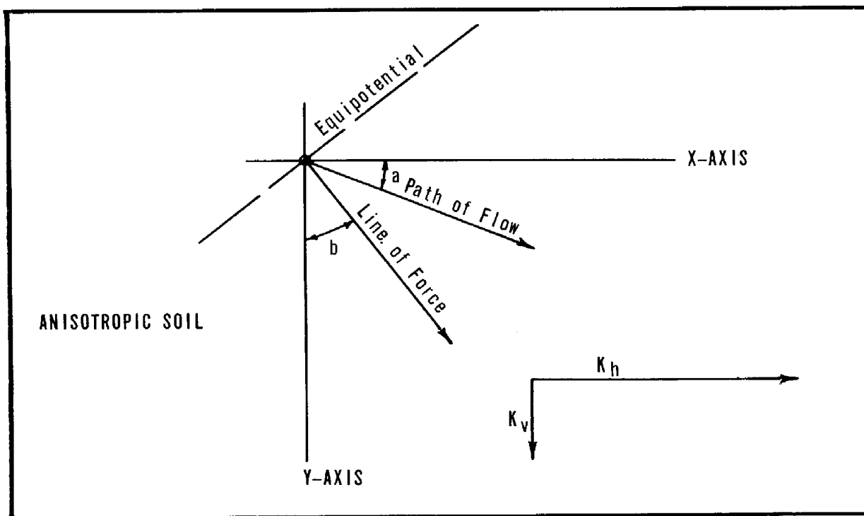
Figure 1-6, Flow direction in anisotropic soil
