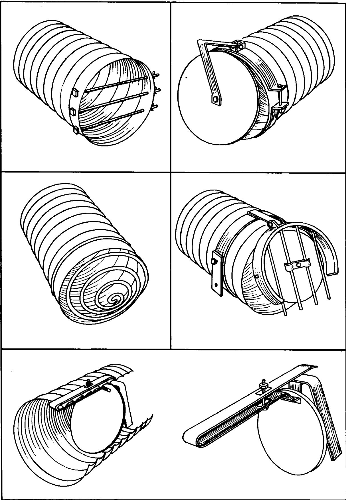
Figure 4-41, Rodent protection for outlet pipe
