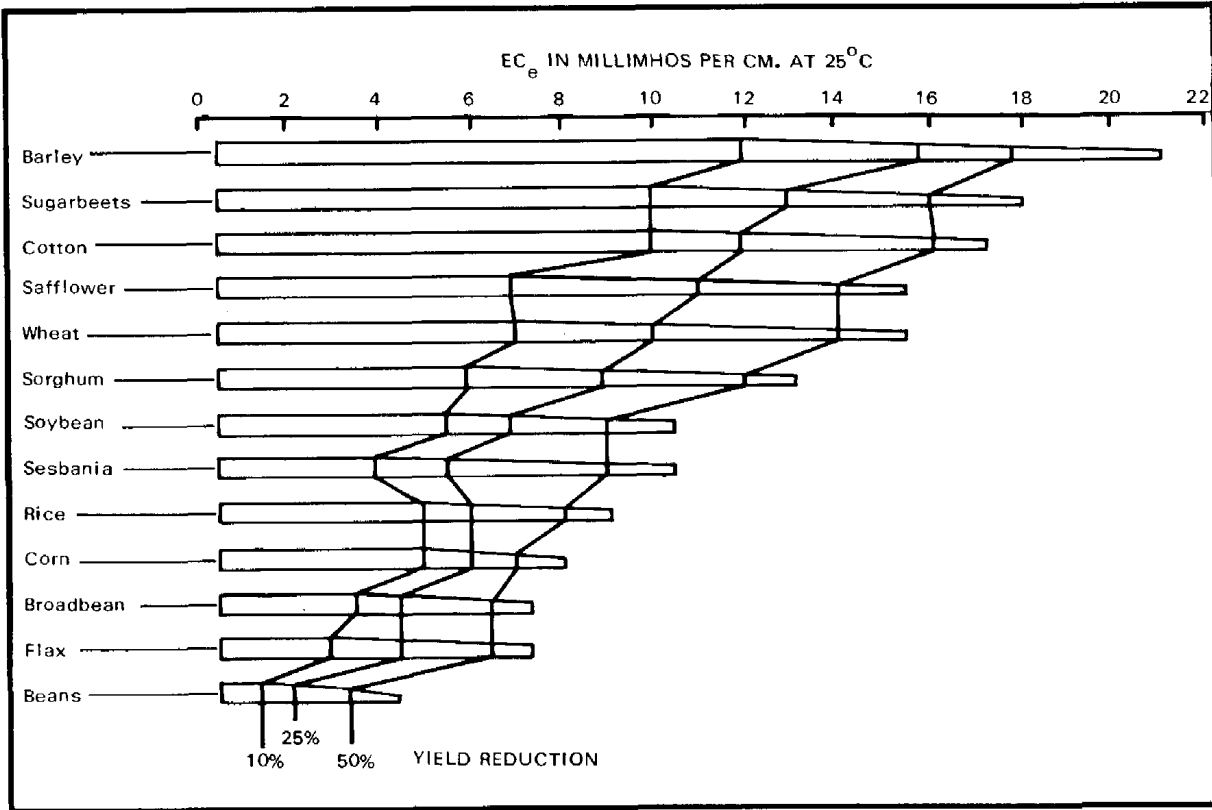
Figure 4-1a, Salt tolerance of field crops
