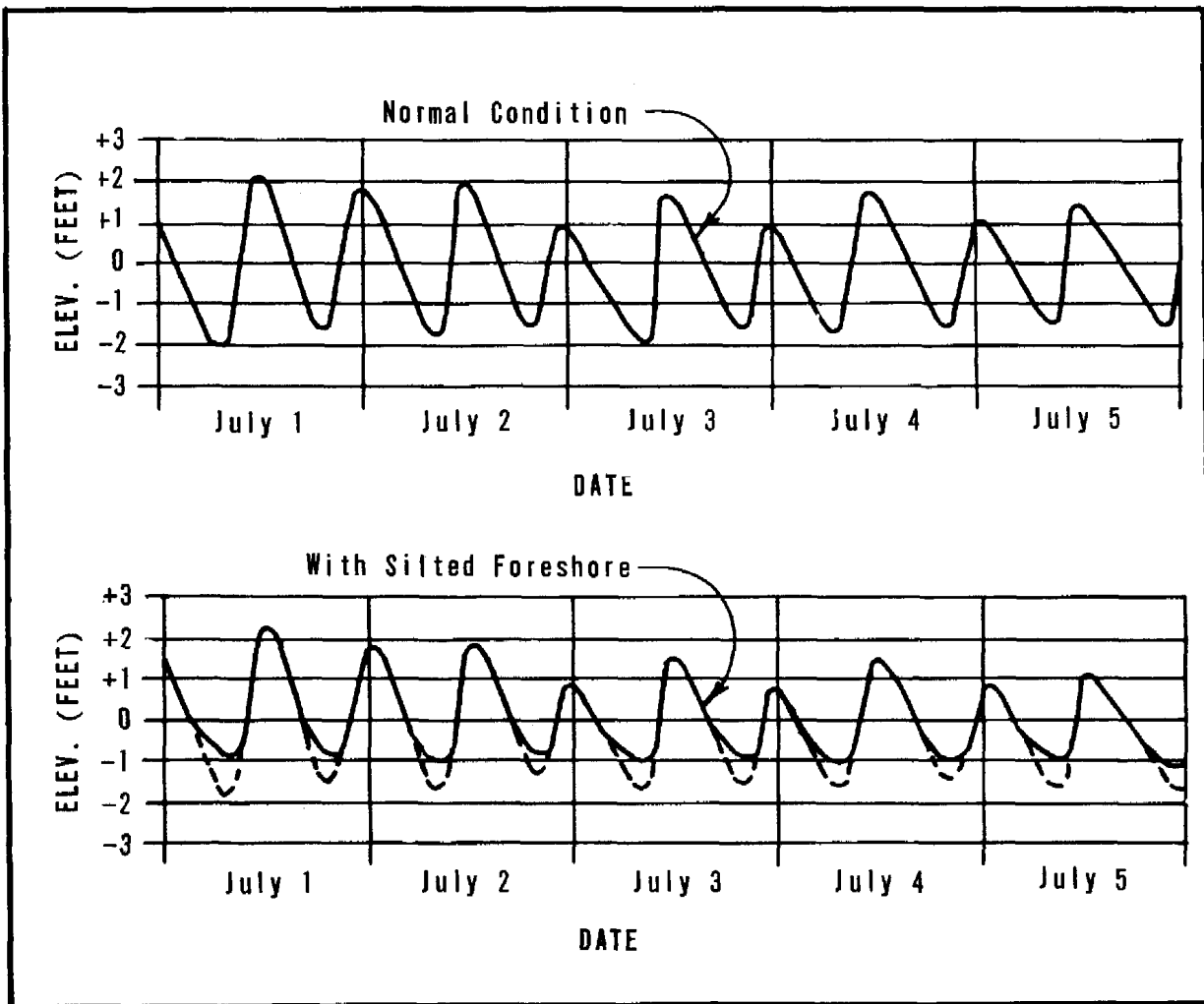
Figure 9-2, Typical estuary tides
