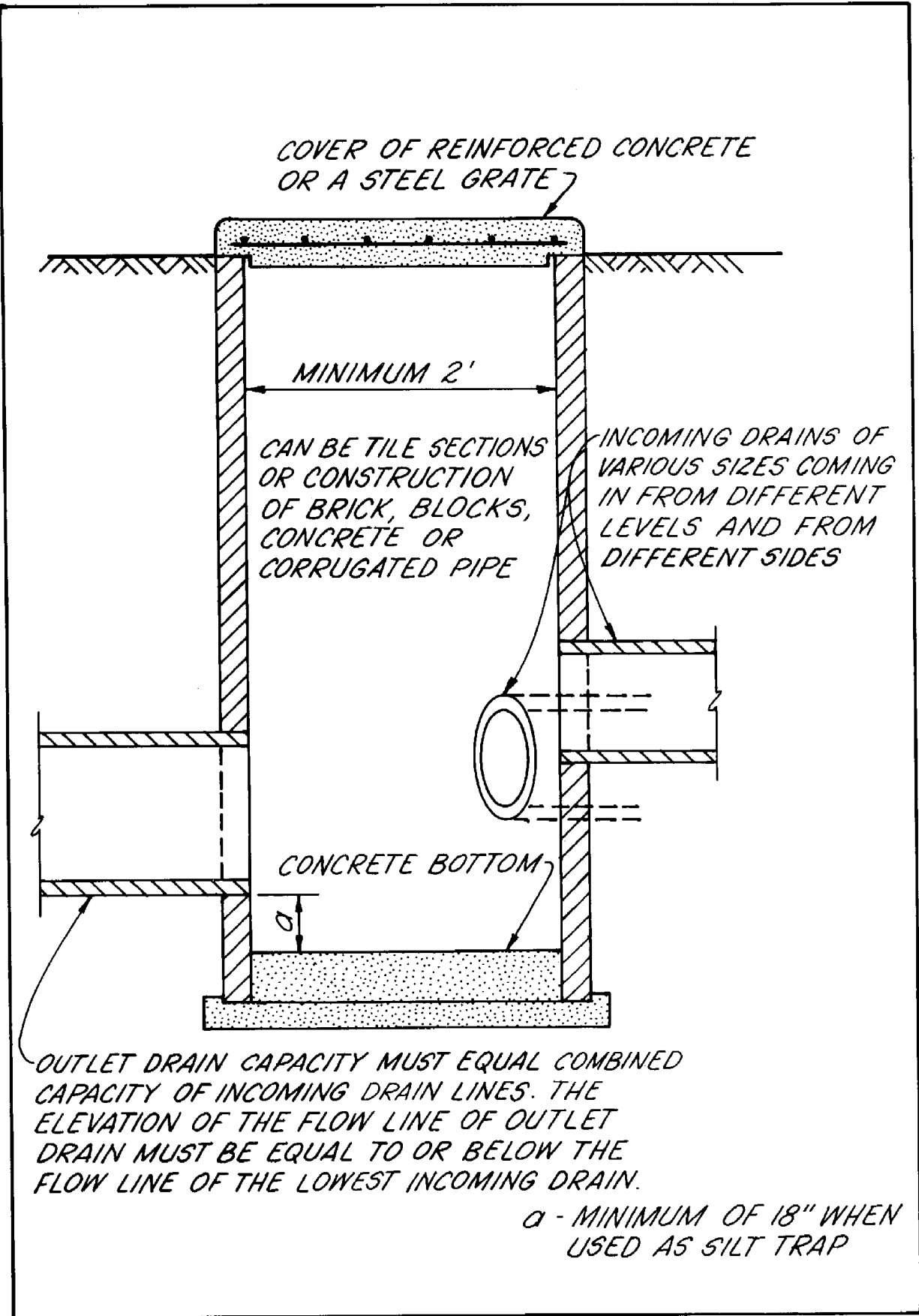
Figure 4-42, Junction box for drains
