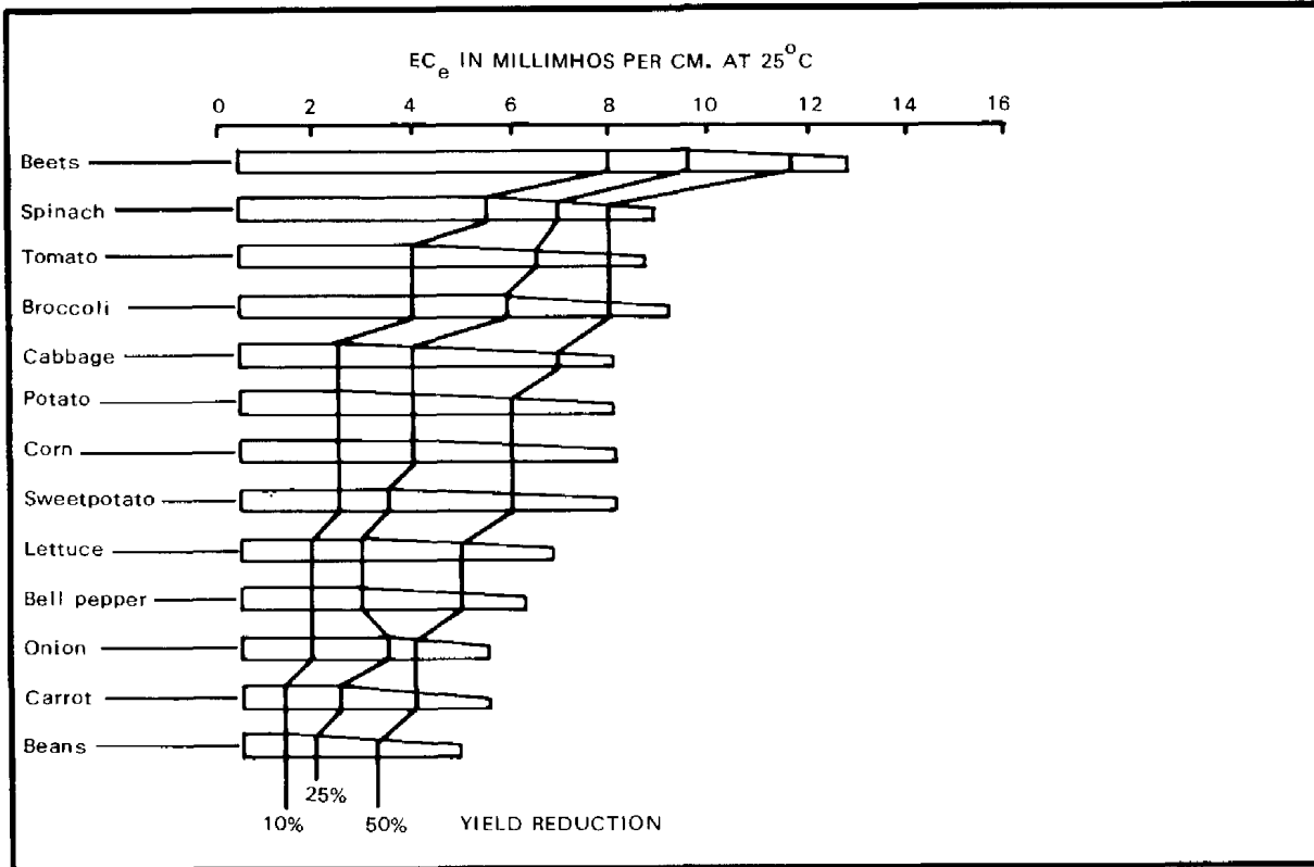
Figure 4-1b, Salt tolerance of vegetable crops
