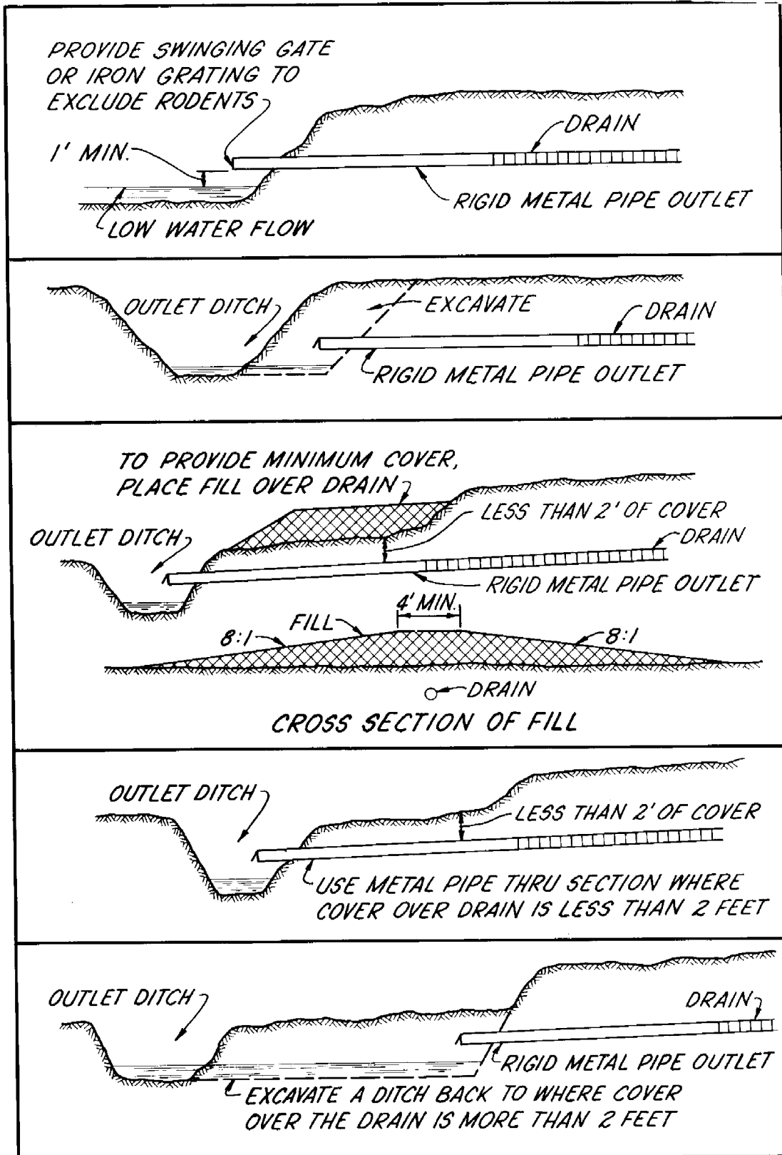
Figure 4-40, Drain outlets
