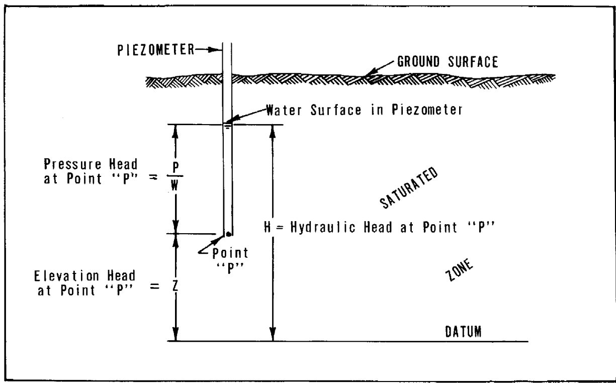
Figure 1-1, Illustration of hydraulic head
