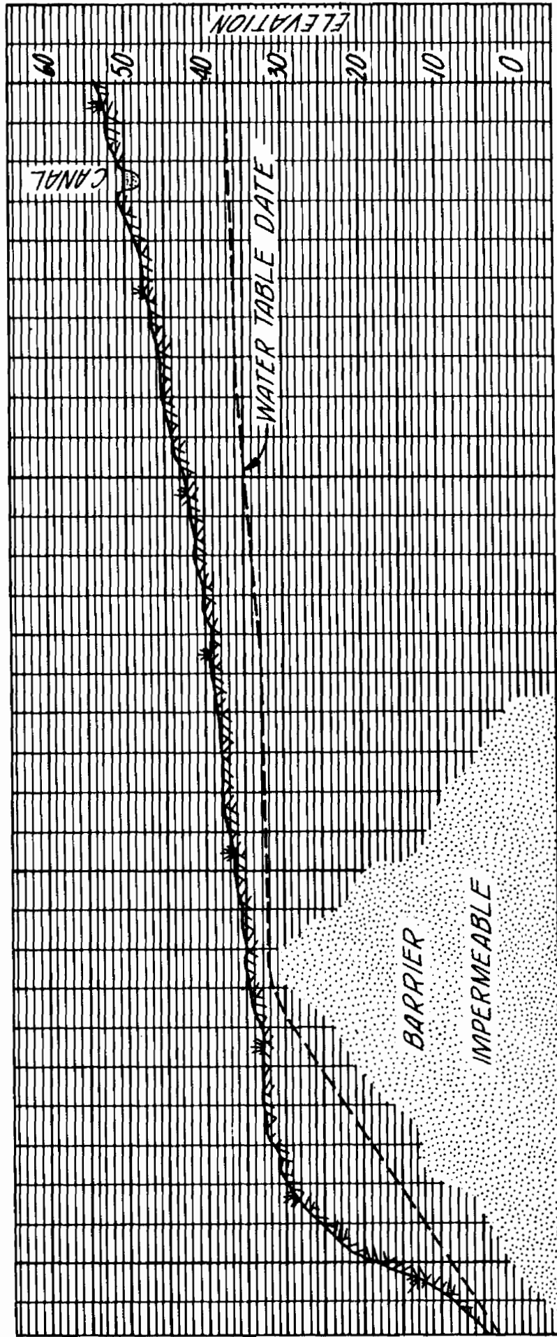
Figure 4-8, Profile section A-A, Figure 4-7
