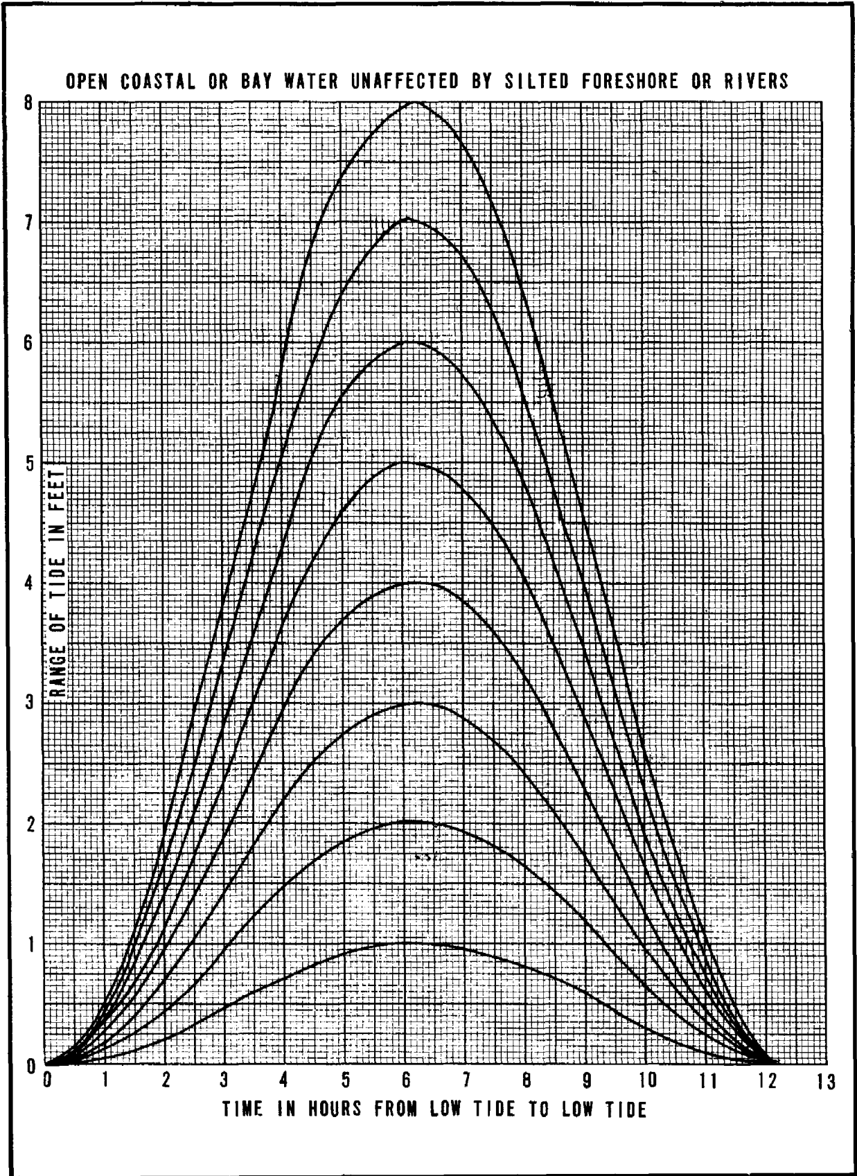
Figure 9-3, Theoretical tide curves
