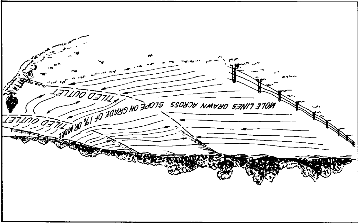
Figure 4-33, Mole drainage system on sloping land
