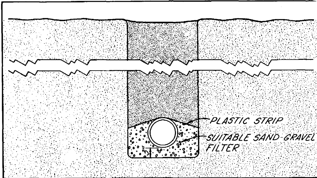
Figure 4-38, Filter installation
