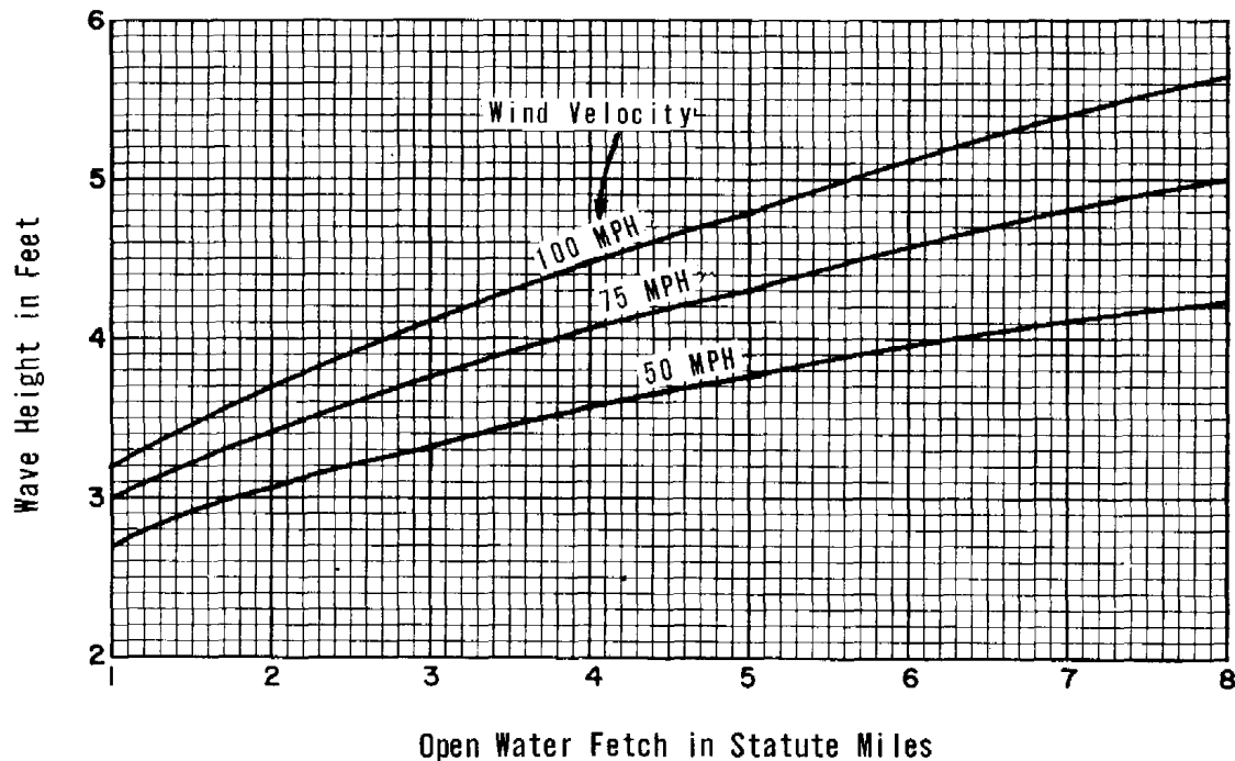
Figure 6-2, Wave height curves
