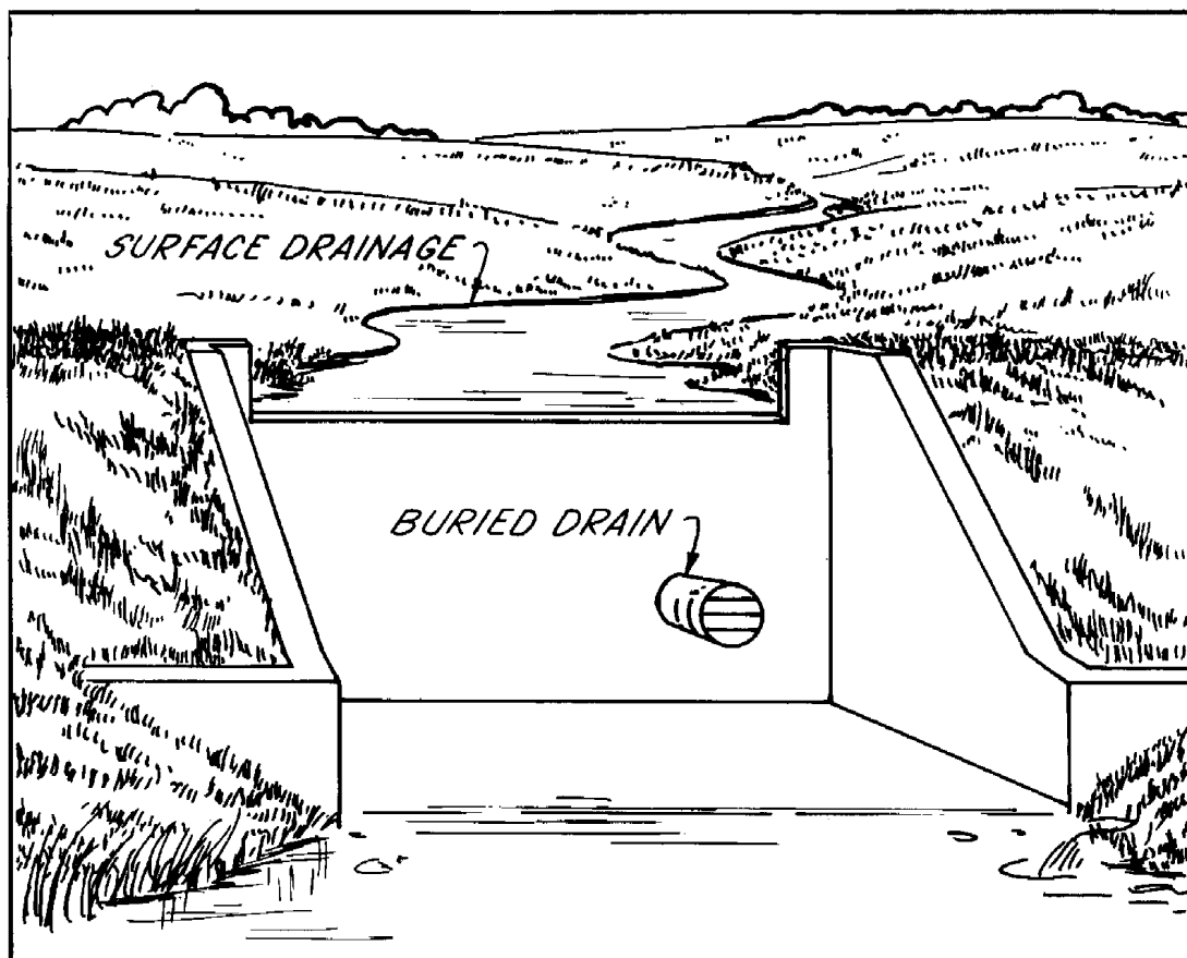
Figure 4-39, Outlet protection
