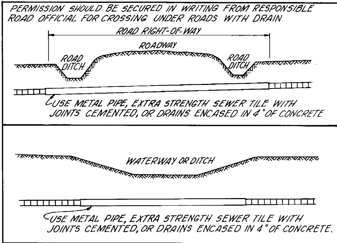
Figure 4-48, Drain crossings
