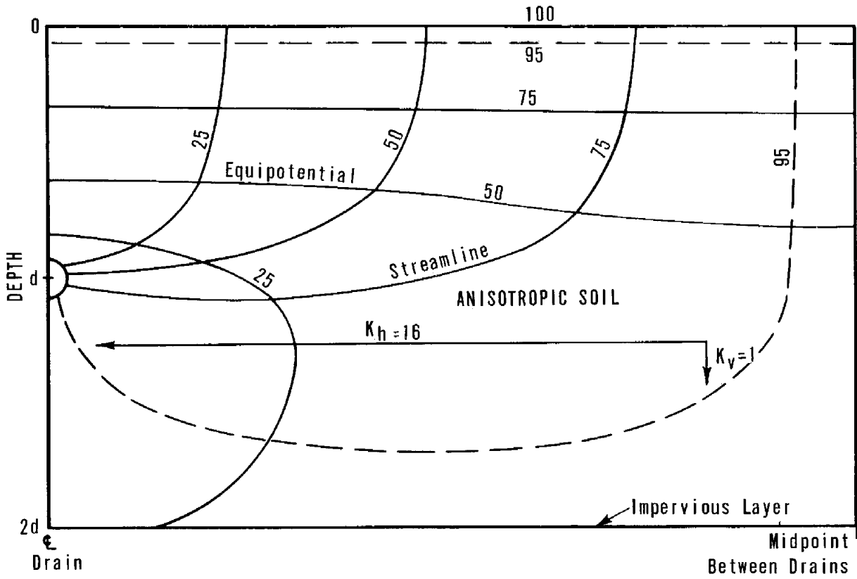
Figure 1-7, Streamlines and equipotentials
