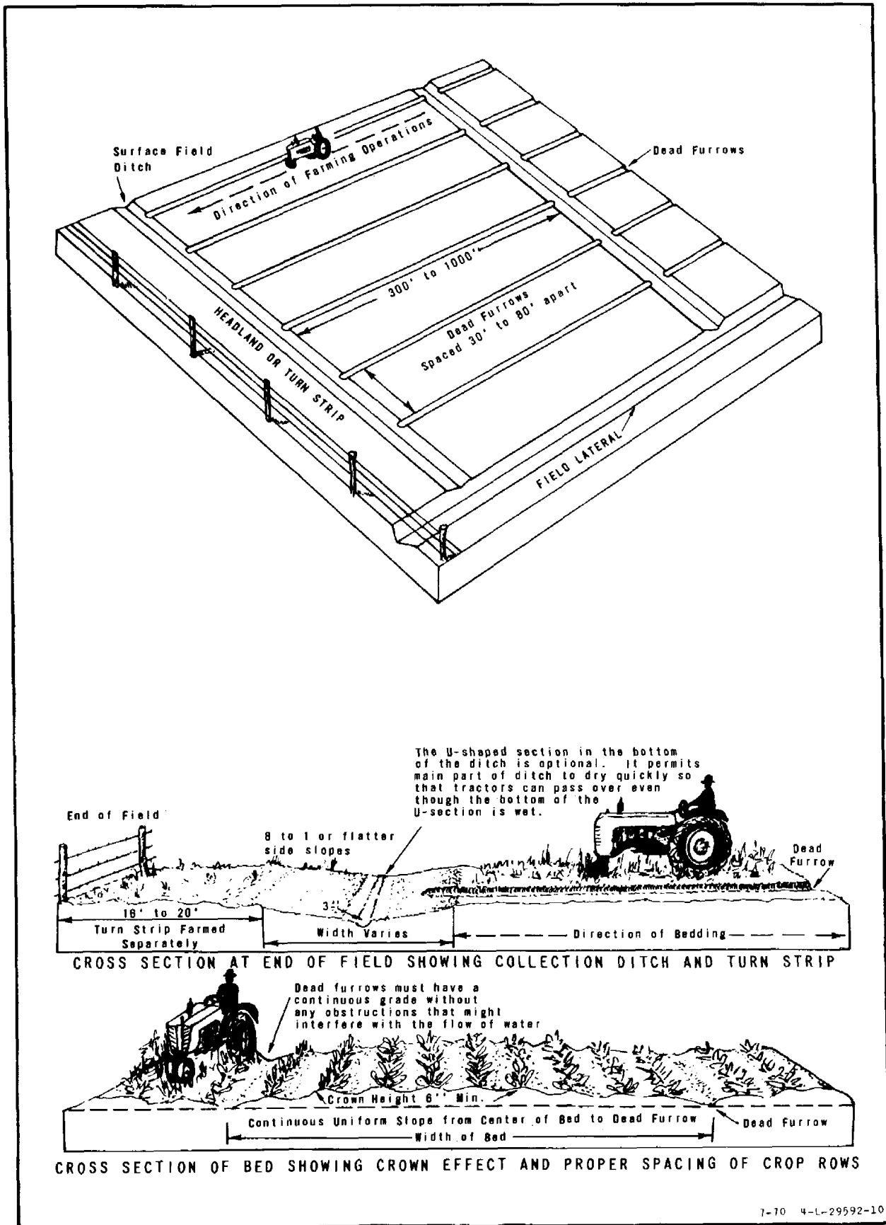
Figure 3-11, Bedding (lands or corrugations)
