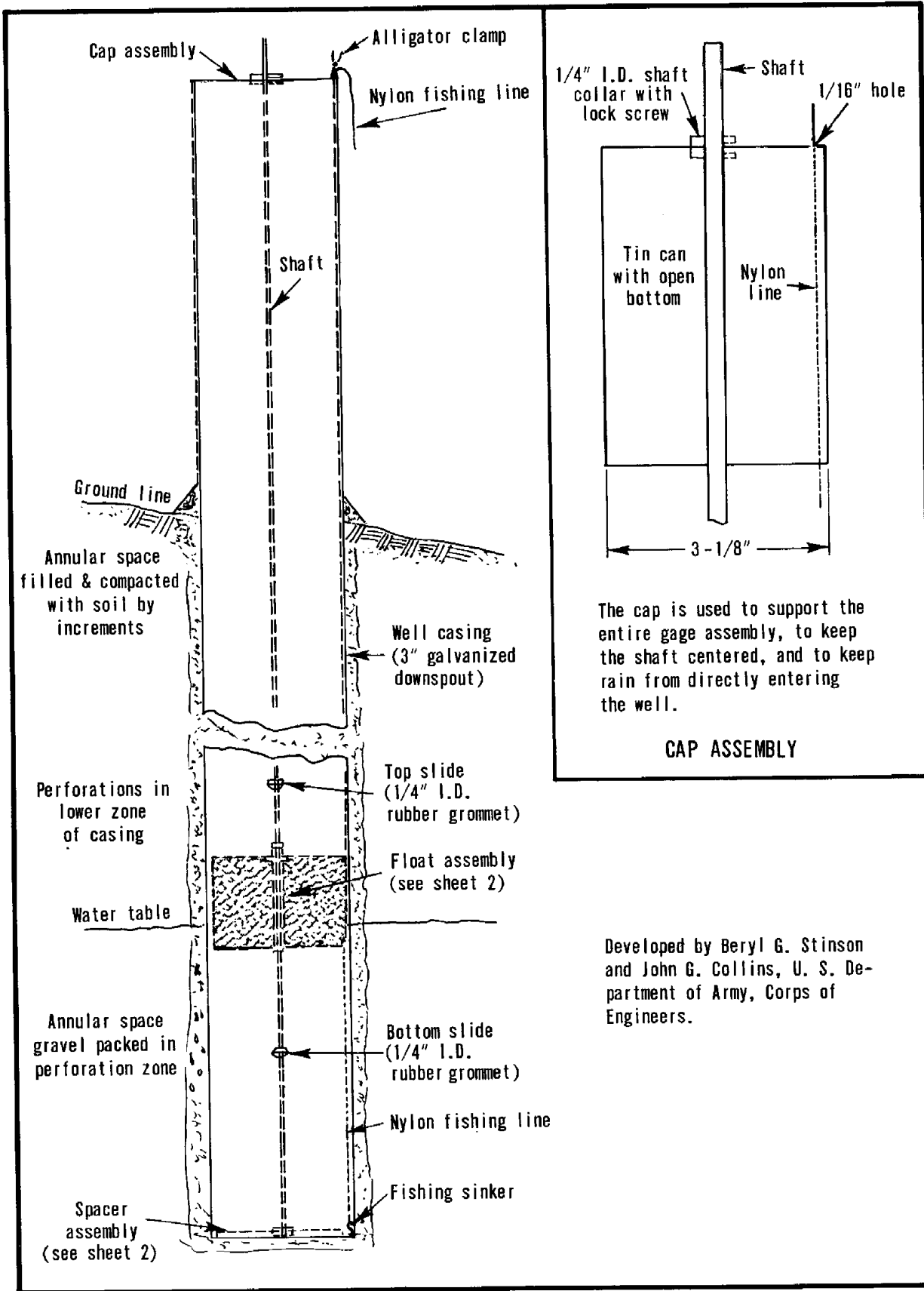
Figure 2-9, Max-min well gage
