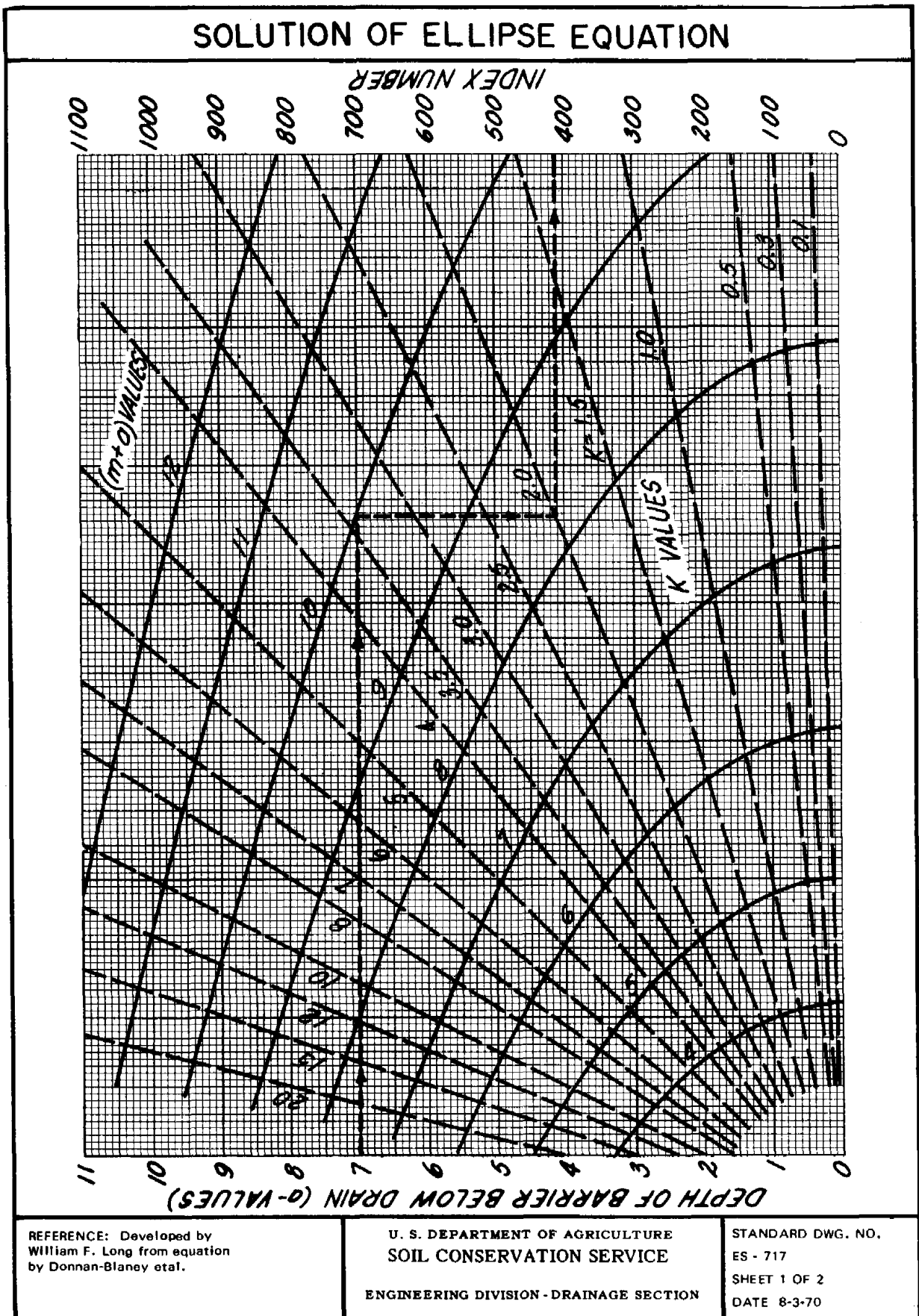
Figure 4-28, Solution of ellipse equation
