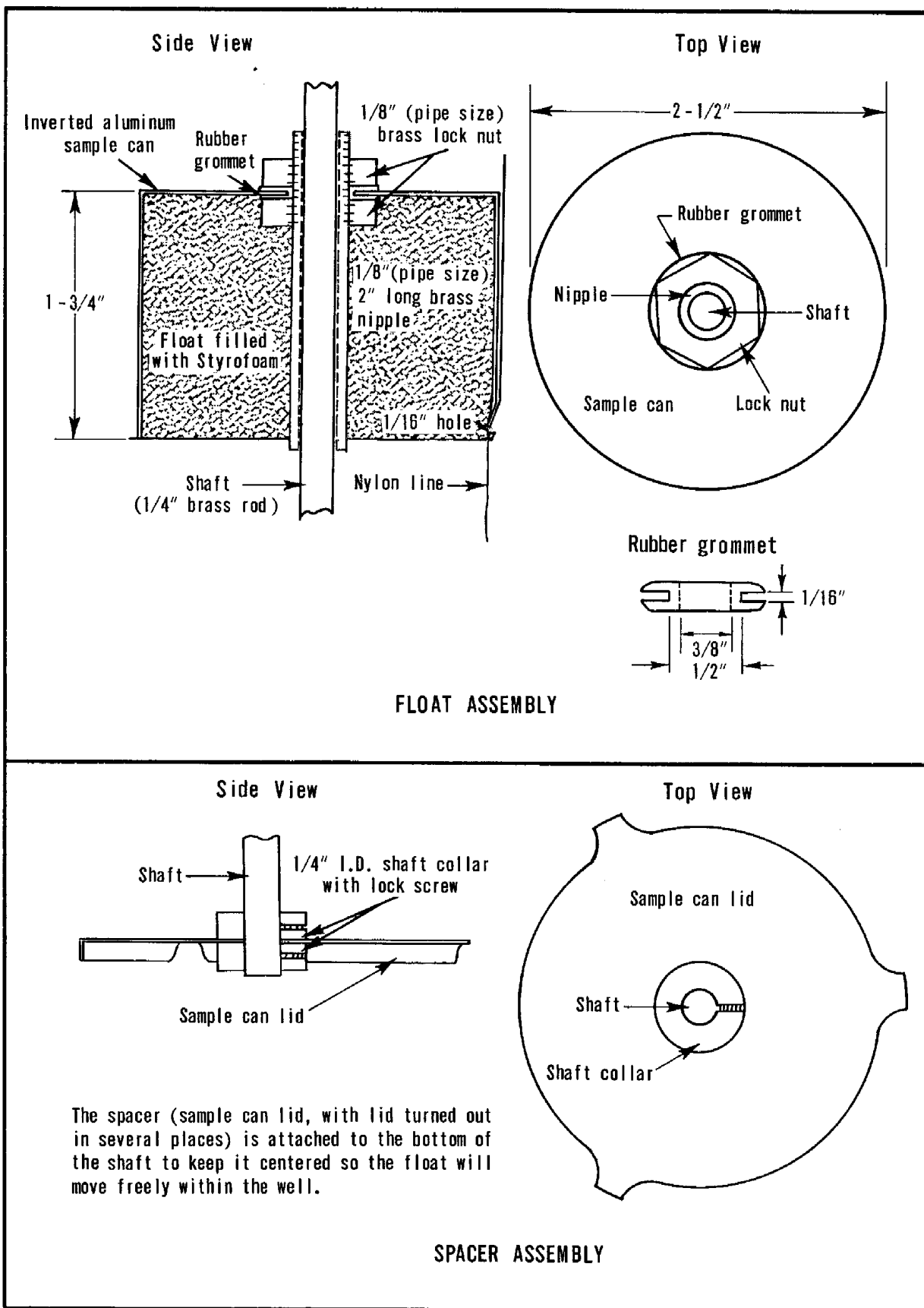
Figure 2-9--sheet 2 of 2, Max-min well gage
