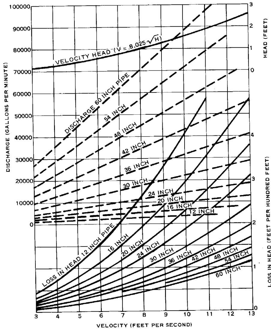
VELOCITY HEAD, DISCHARGE, AND FRICTION-HEAD LOSS IN RIVETED STEEL PIPES
