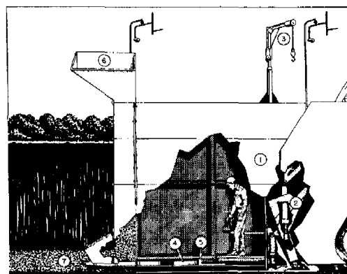
Hydraulic ram in shoring cage
