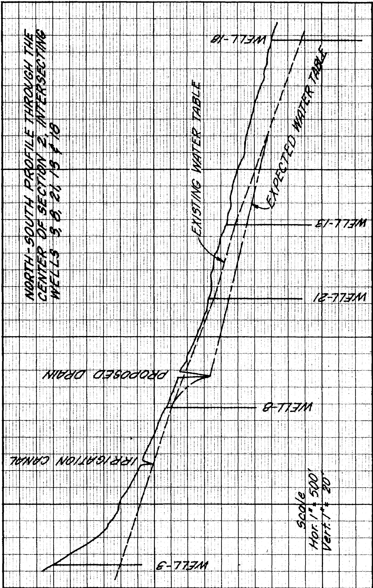
Figure 4-20, Profile--Figure 4-19
