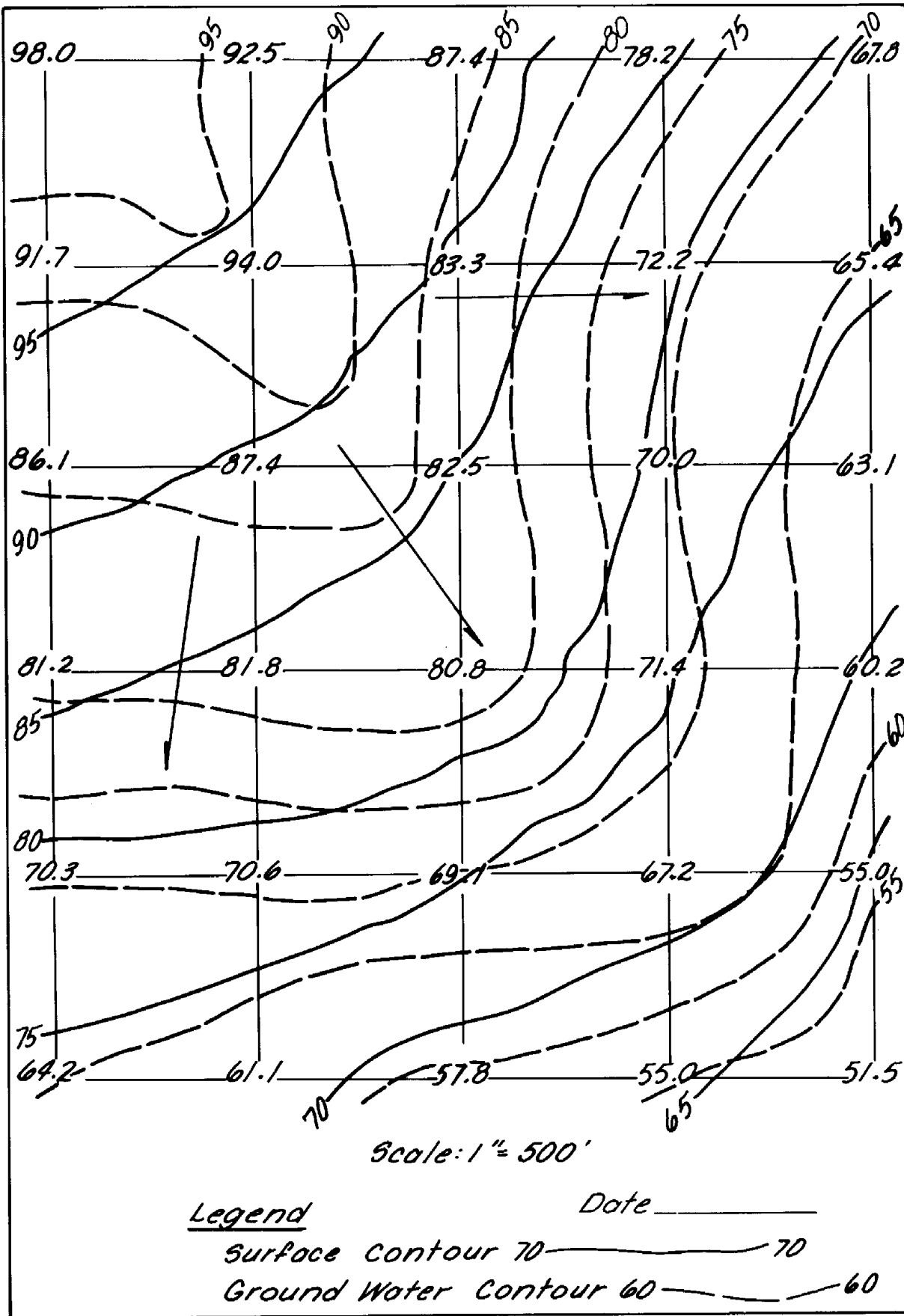
Figure 4-5, Typical ground-water contour map
