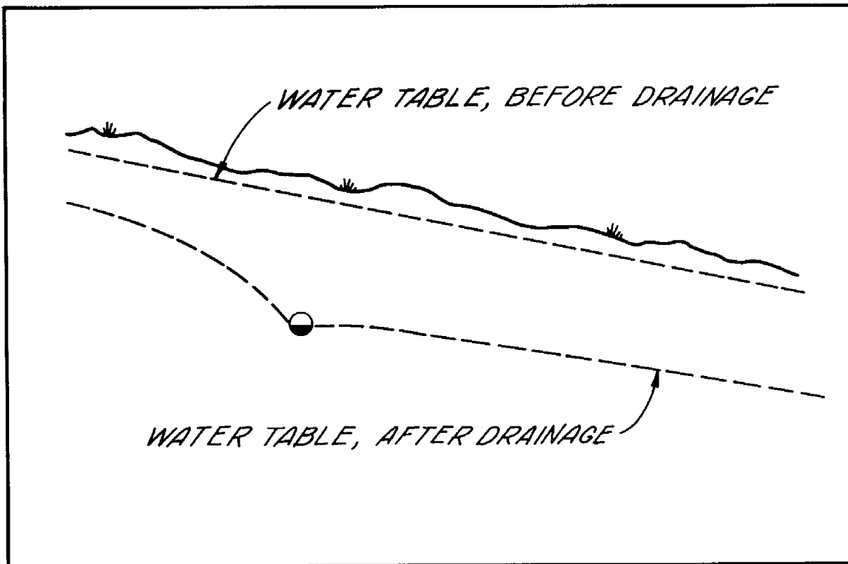
Figure 4-25b, Interception drain
