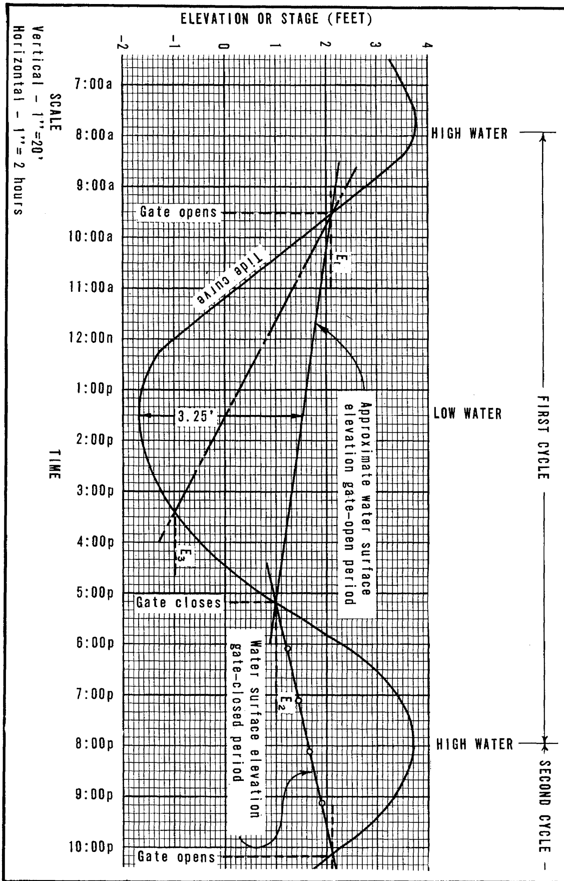
Figure 9-4, Tide curve
