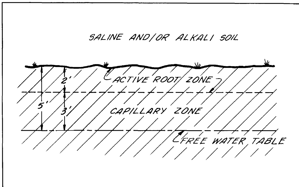
Figure 4-2a, Soil profile showing high capillarity
