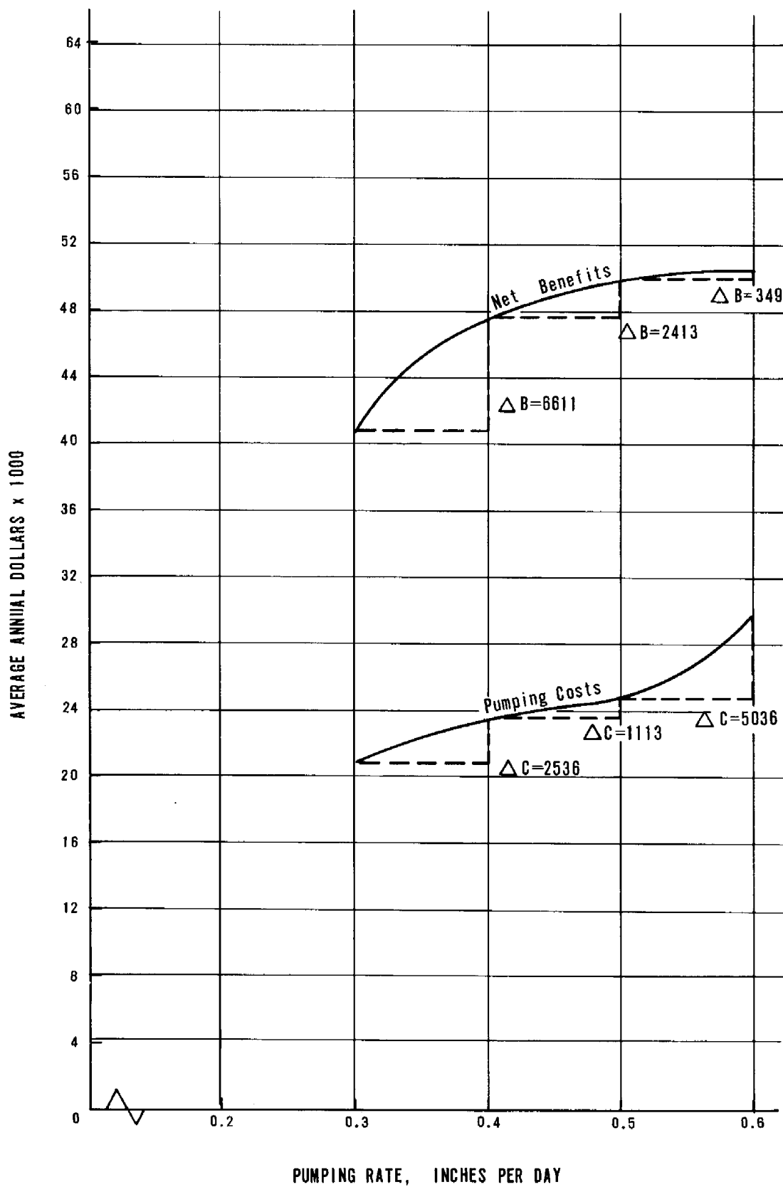
Figure 7A-10, Cost-benefit relationship at various pumping rates
