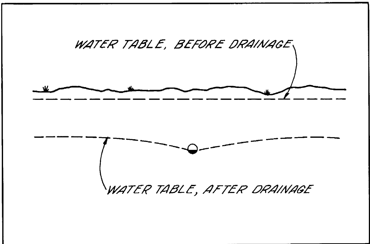
Figure 4-24b, Relief drain
