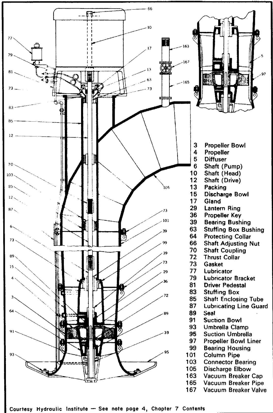
Figure 7-2, Propeller or axial flow pump
