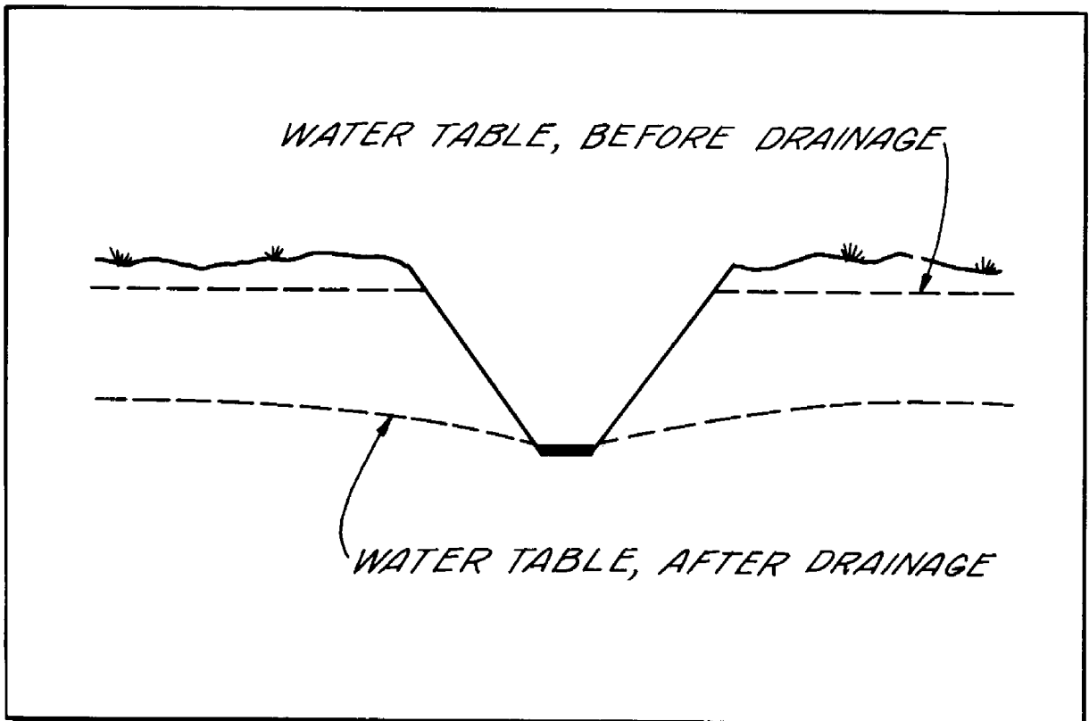
Figure 4-24a, Relief ditch
