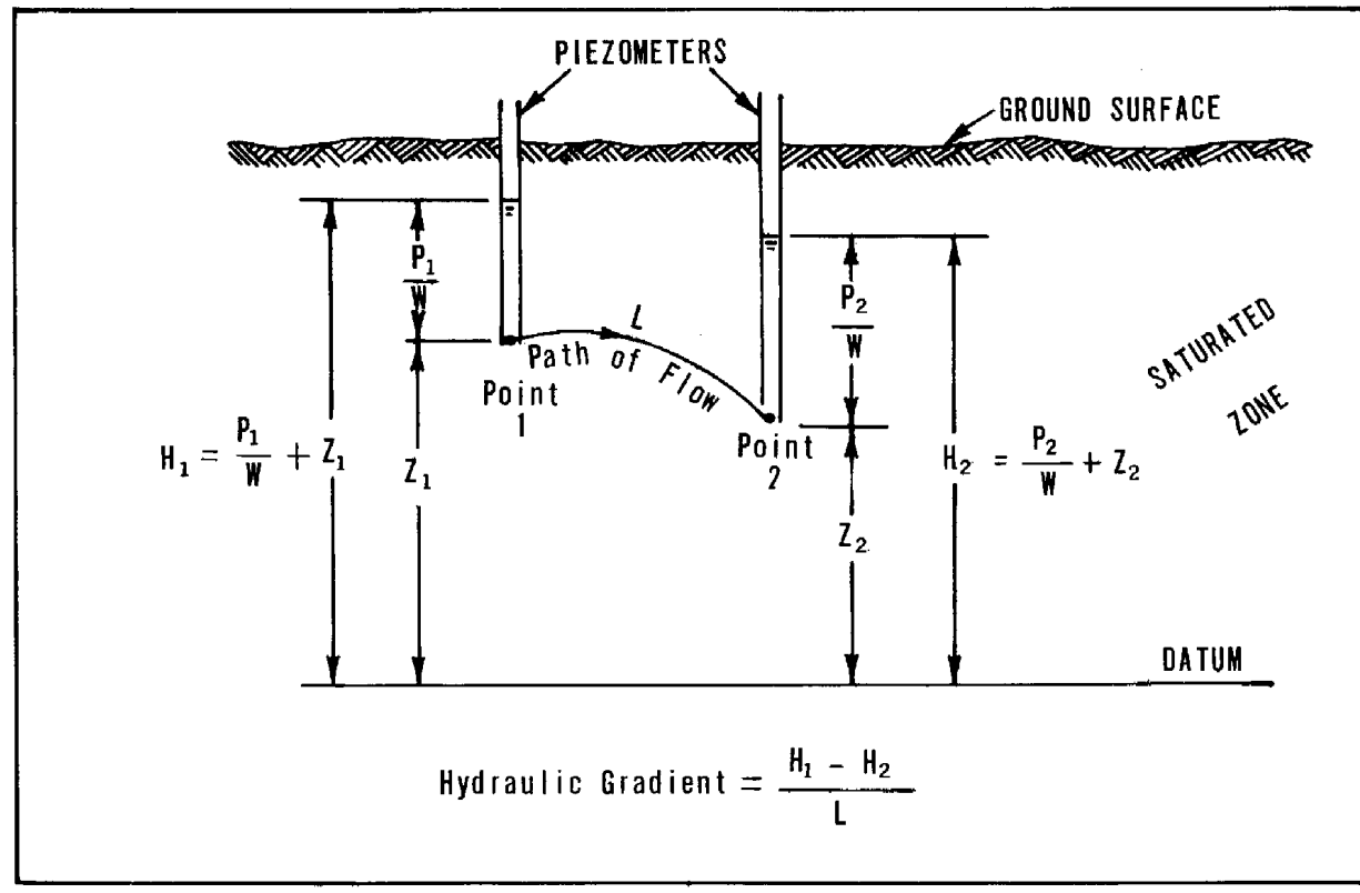
Figure 1-2, Illustration of hydraulic gradient
