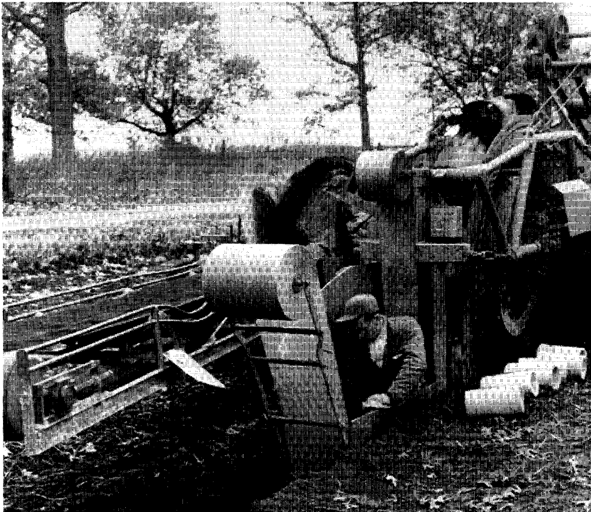
Installing fiber mat base and filter
