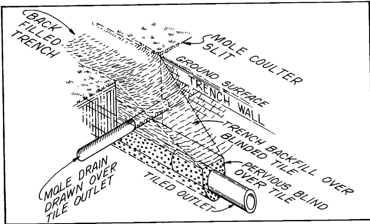
Figure 4-34, Buried drain outlet for mole drain
