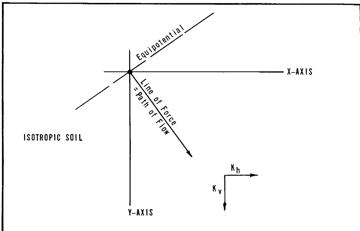
Figure 1-5, Flow direction in isotropic soil
